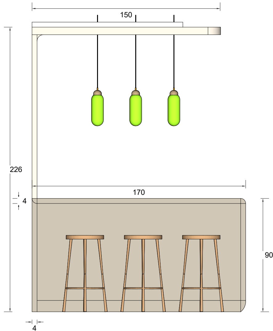
FRONT ELEVATION BREAKFAST COUNTER
